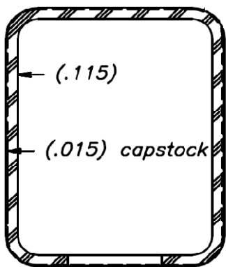
2.10" x 2.661" Rail
